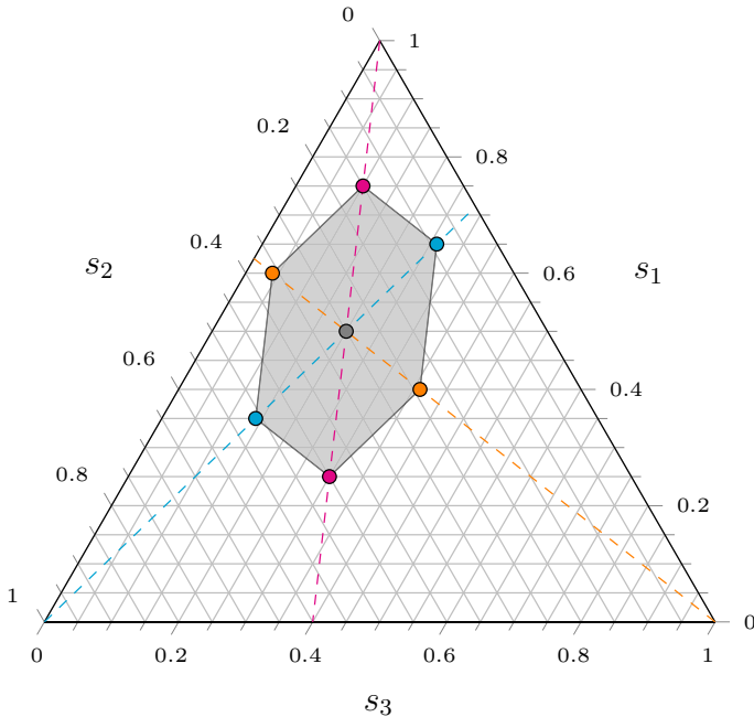
Fig. 1 The set of priors for S = \{s_1, s_2, s_3\} and \mu = (.5, .3, .2) , and \lambda = 1
